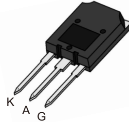
TO-247S (non-Insulated) (70PTxxDS)
